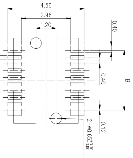
RECOMMENDED PCB PATTERN LAYOUT
